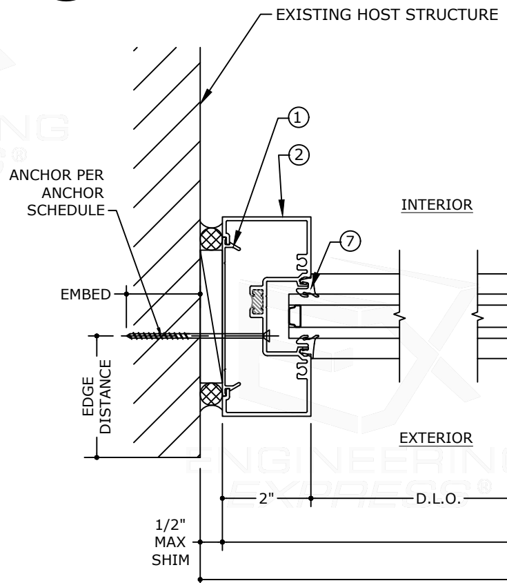
D TYPICAL JAMB DETAIL 4" = 1'-0" HORIZONTAL SECTION
