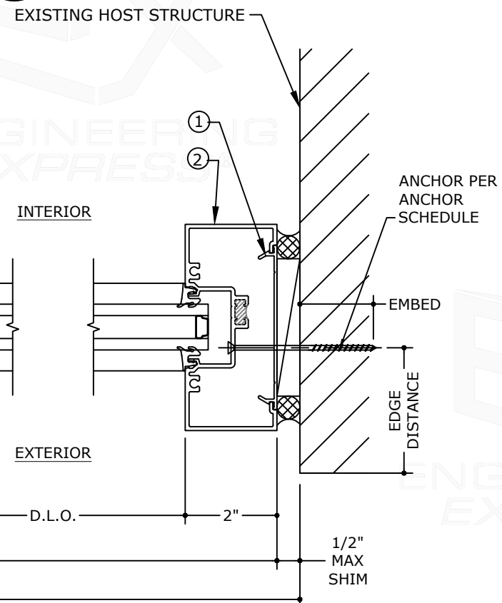
F TYPICAL JAMB DETAIL 4" = 1'-0" HORIZONTAL SECTION
